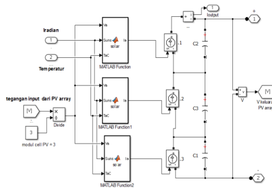
Gambar 13. Model PV array
