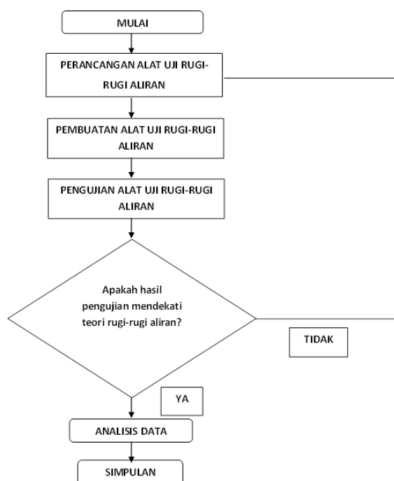
Gambar 3. Diagram Alir
